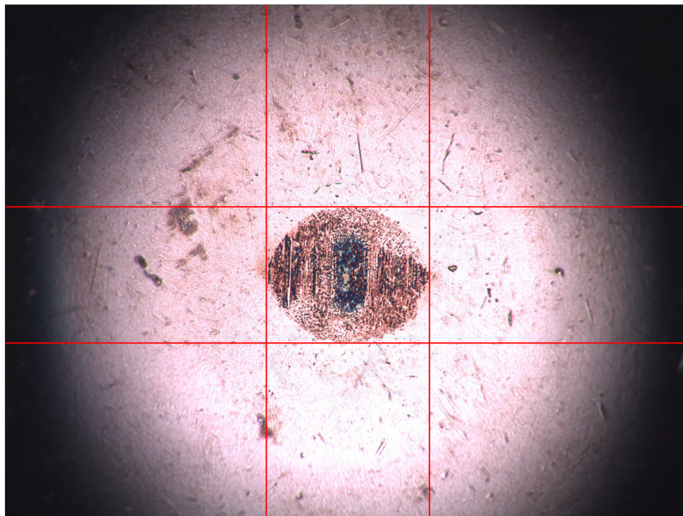
Microscope wear scar measurement 1 of 1 measured by LC on 2/11/2009 at 4:21 PM
