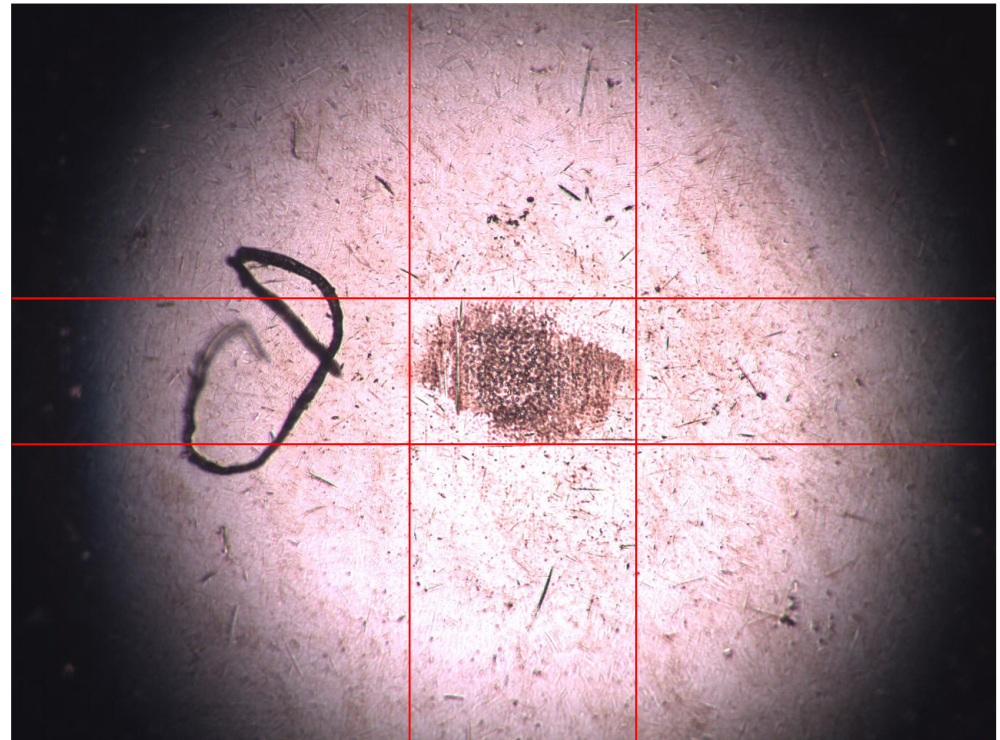
Microscope wear scar measurement 1 of 1 measured by JA on 2/13/2009 at 9:45 AM
